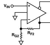
Figure 5. Typical Circuit with \beta_1 = 0
