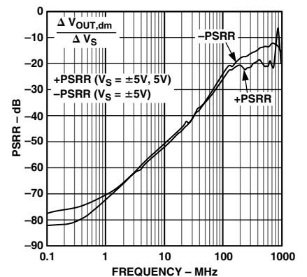
TPC 49. PSRR vs. Frequency
