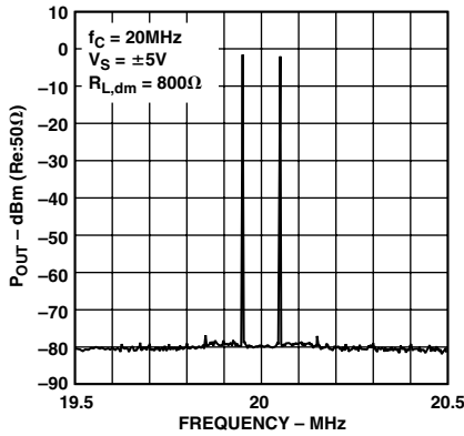
TPC 35. Intermodulation Distortion, G = 1
