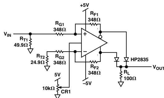
Figure 19. Full-Wave Rectifier
